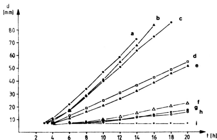
Fig. 2. Swarming rates of (a) Serratia marcescens , (b) its mutant Sm1, (c) Salmonella typhimurium LT2, (d) Enterobacter aerogenes , (e) Salmonella typhimurium 7-73, (f) Proteus mirabilis , (g) Proteus vulgaris , (h) Serratia marcescens Sm6, (i) Azospirillum brasilense .
