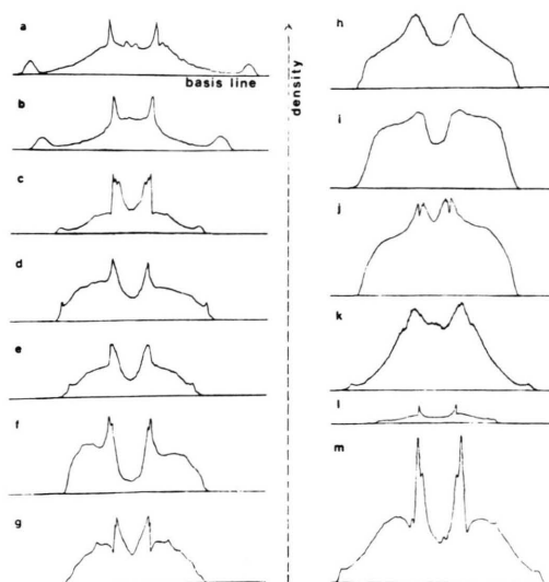
Fig. 1. Densitograms of the swarming zones of (a) Serratia marcescens , (b) and (c) its mutants Sm1 and Sm6, (d) Salmonella typhimurium LT2, (e) and (f) its mutants 7-73 and TA 1535, (g) Enterobacter aerogenes , (h) Pseudomonas acidovorans , (i) Pseudomonas aureofaciens , (j) Pseudomonas diminuta , (k) Azospirillum brasilense , (l) Proteus mirabilis , (m) Proteus vulgaris . These densitograms were taken, when the diameters of the spreading zone amounted to about 30 mm. The basis line represents the density of the medium.
